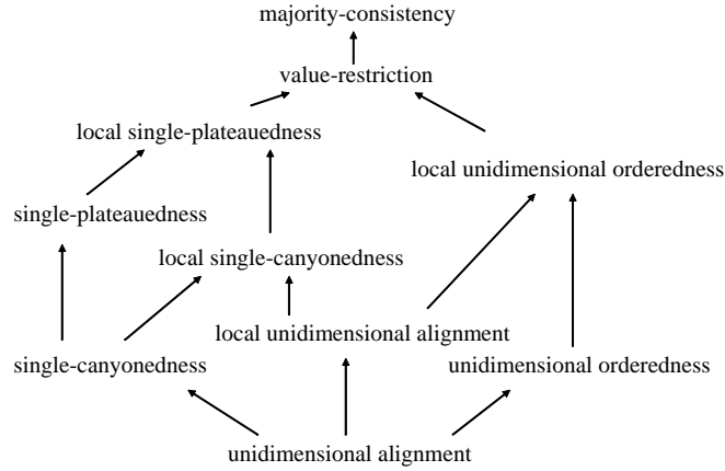
Figure 3: The logical relationships between the domain-restriction conditions for profiles of consistent judgment sets
